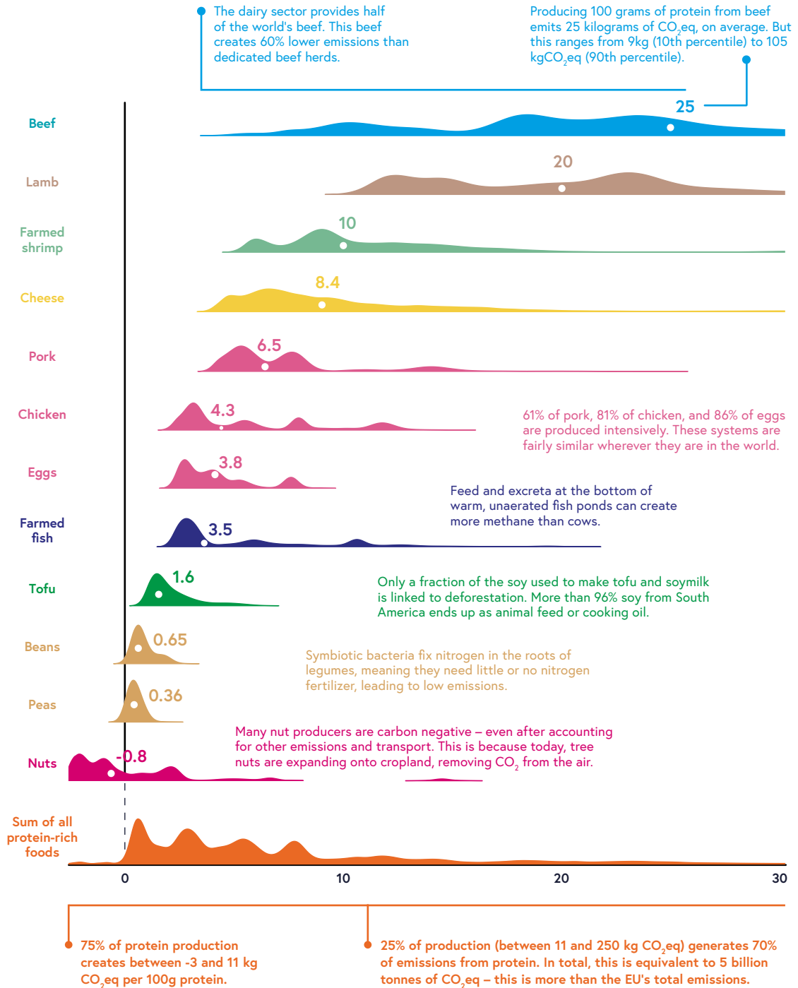
Greenhouse gas emissions per 100 grams of protein (kilograms of carbon dioxide equivalents; kgCO 2 eq)
